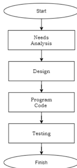
Figure 1 Research Framework
