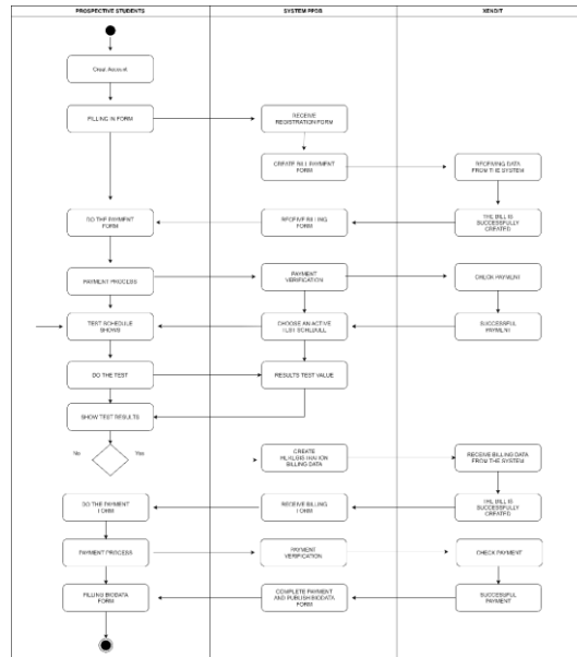
Figure 5. Activity Diagram
