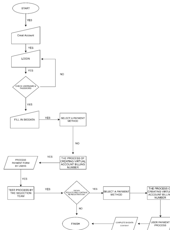
Figure 2. User Flow Chart
