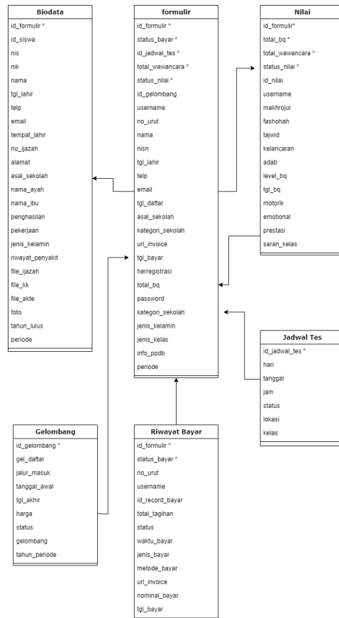
Figure 8. Relationships Between Tables
