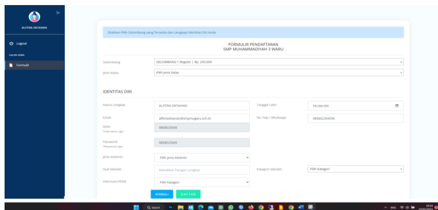
Figure 9. Form Page
