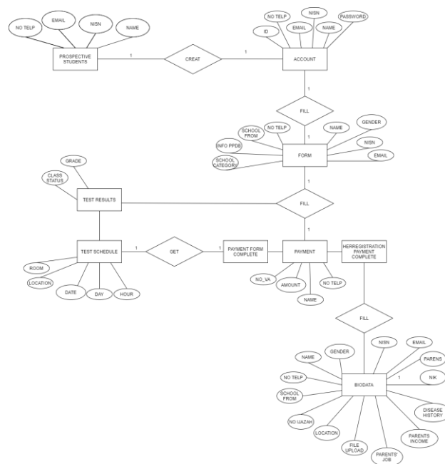
Figure 7. ERD
