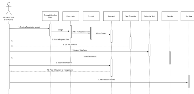
Figure 6. Sequence Diagram
