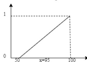
Figure 5. Fuzzy Graph for K2
