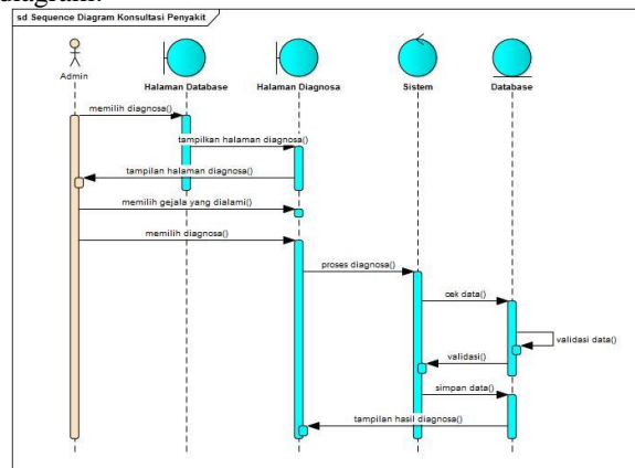
Fig 6. Sequence Diagram
