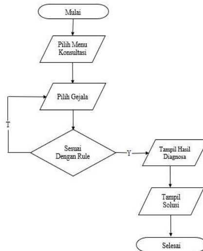
Fig. 1. Algorithm Design
