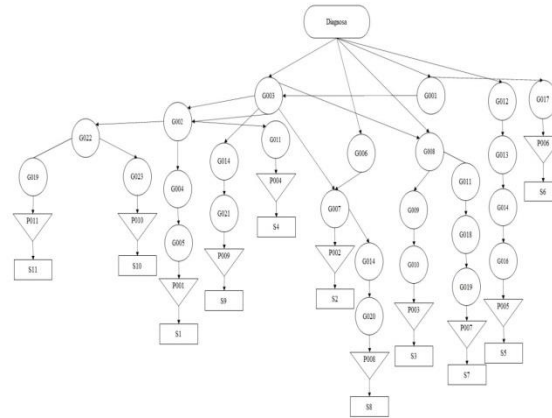
Fig. 2. Decision Tree
