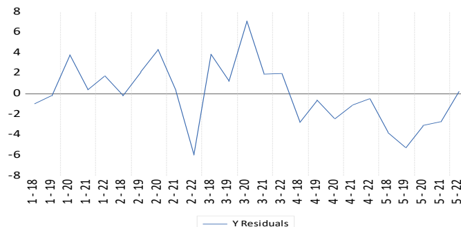
Figure 2. Heteroscedasticity test results
